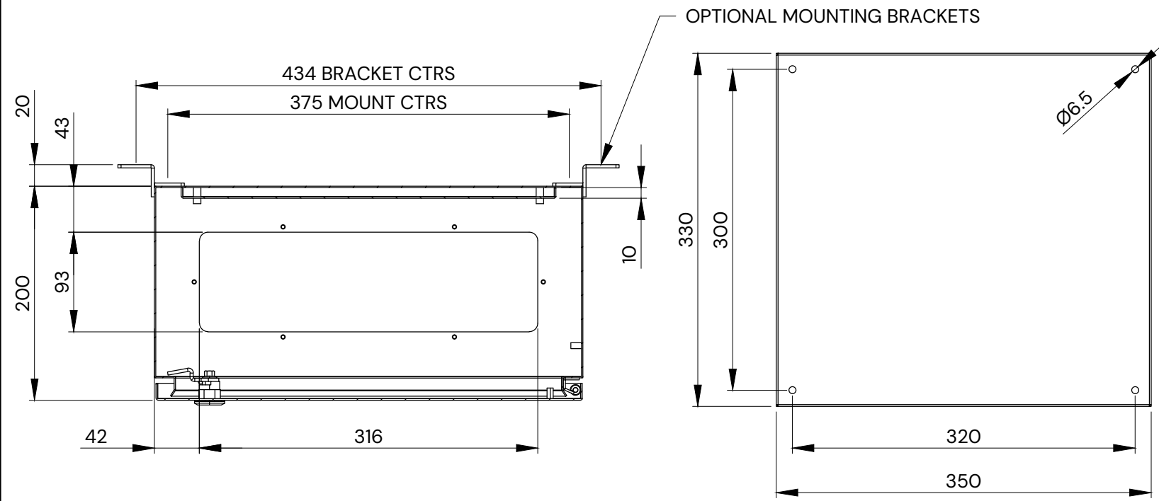
SECTION AW-AW
