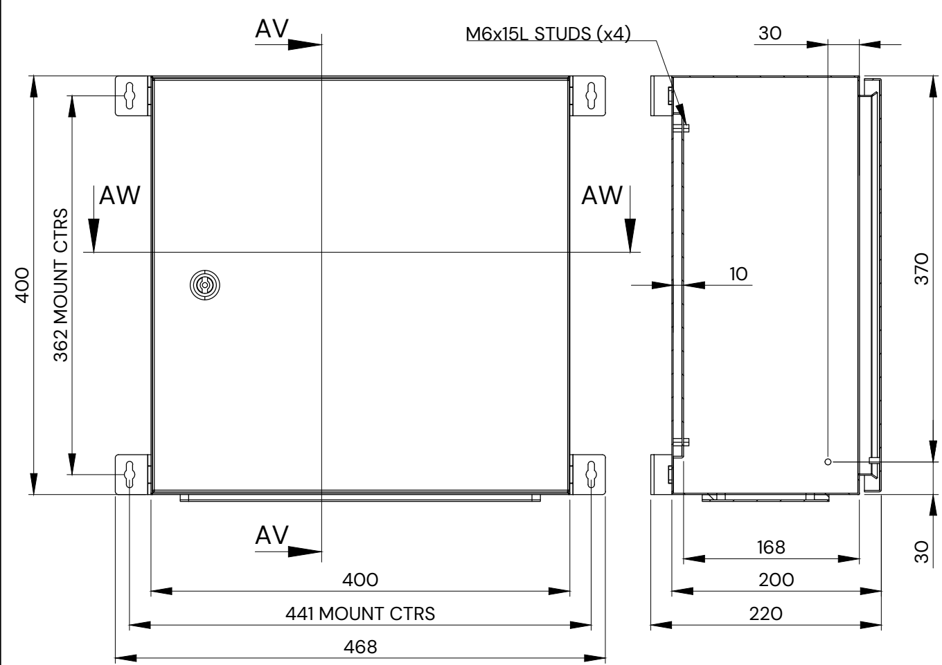
FRONT VIEW
