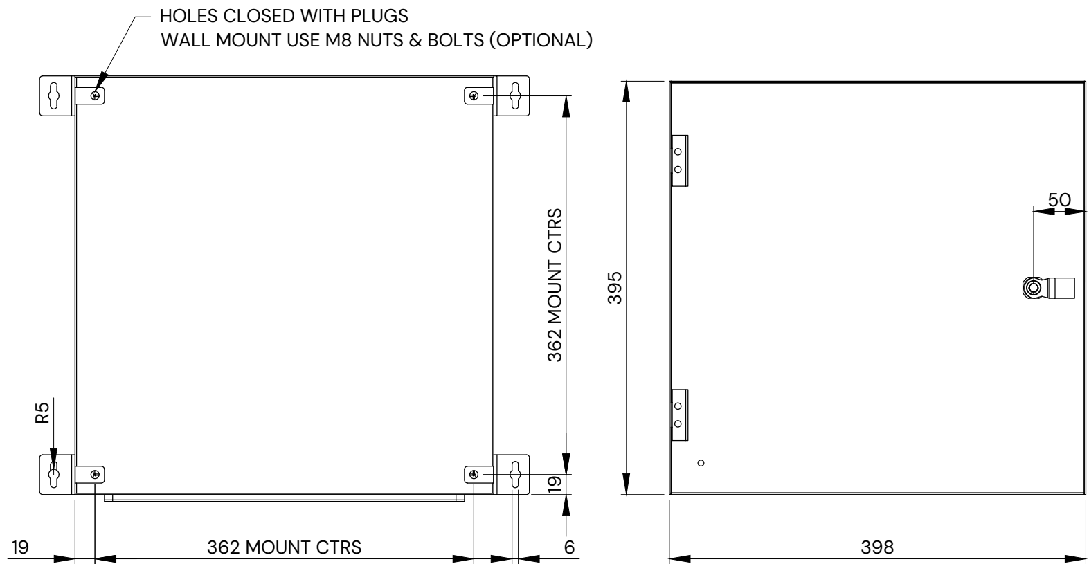
REAR VIEW
