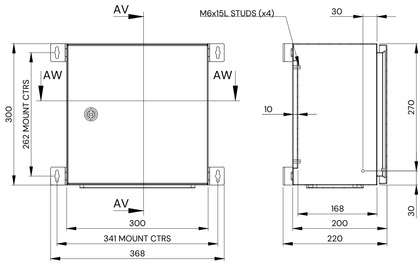
FRONT VIEW
