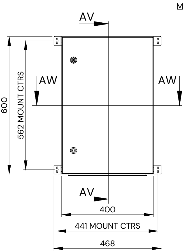
FRONT VIEW
