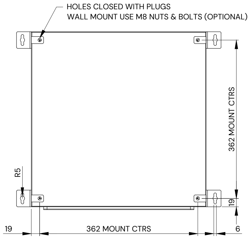
REAR VIEW
